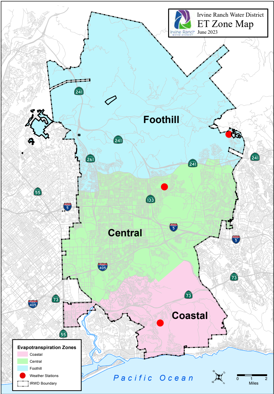
Figure 7. Updated ET zone map for IRWD, dividing the water district into three zones (Coastal, Central and Foothill), and identifying the location of the three IRWD weather stations.
