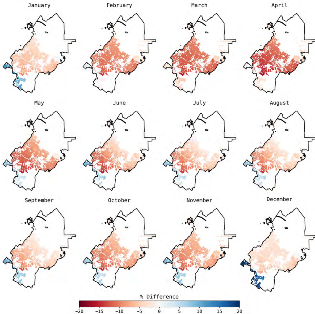
Figure 6. Same as Figure 5 but in percent difference.
