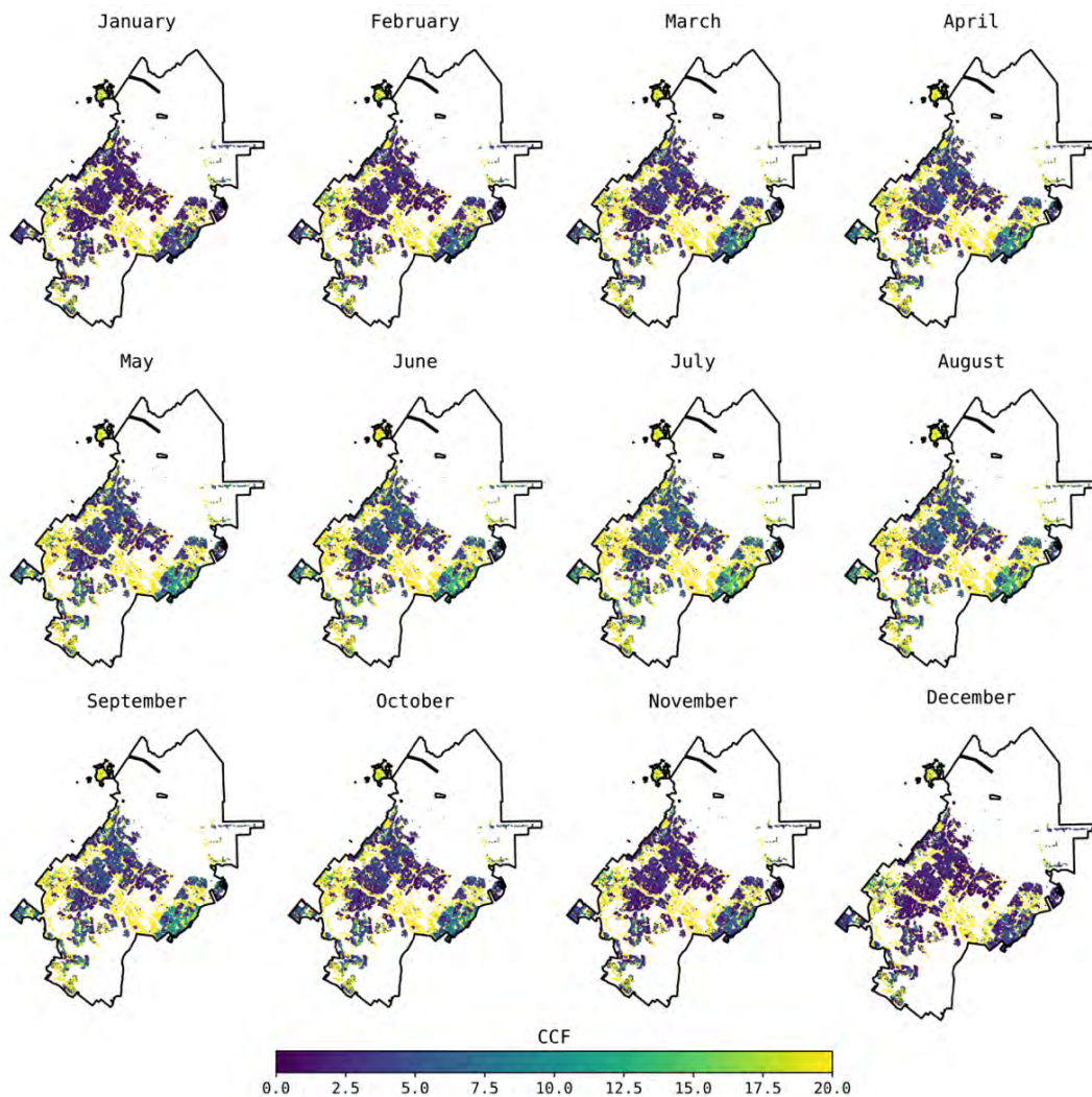
Figure A2. Same as Figure A1 but with the water budget computed using Spatial CIMIS data.
