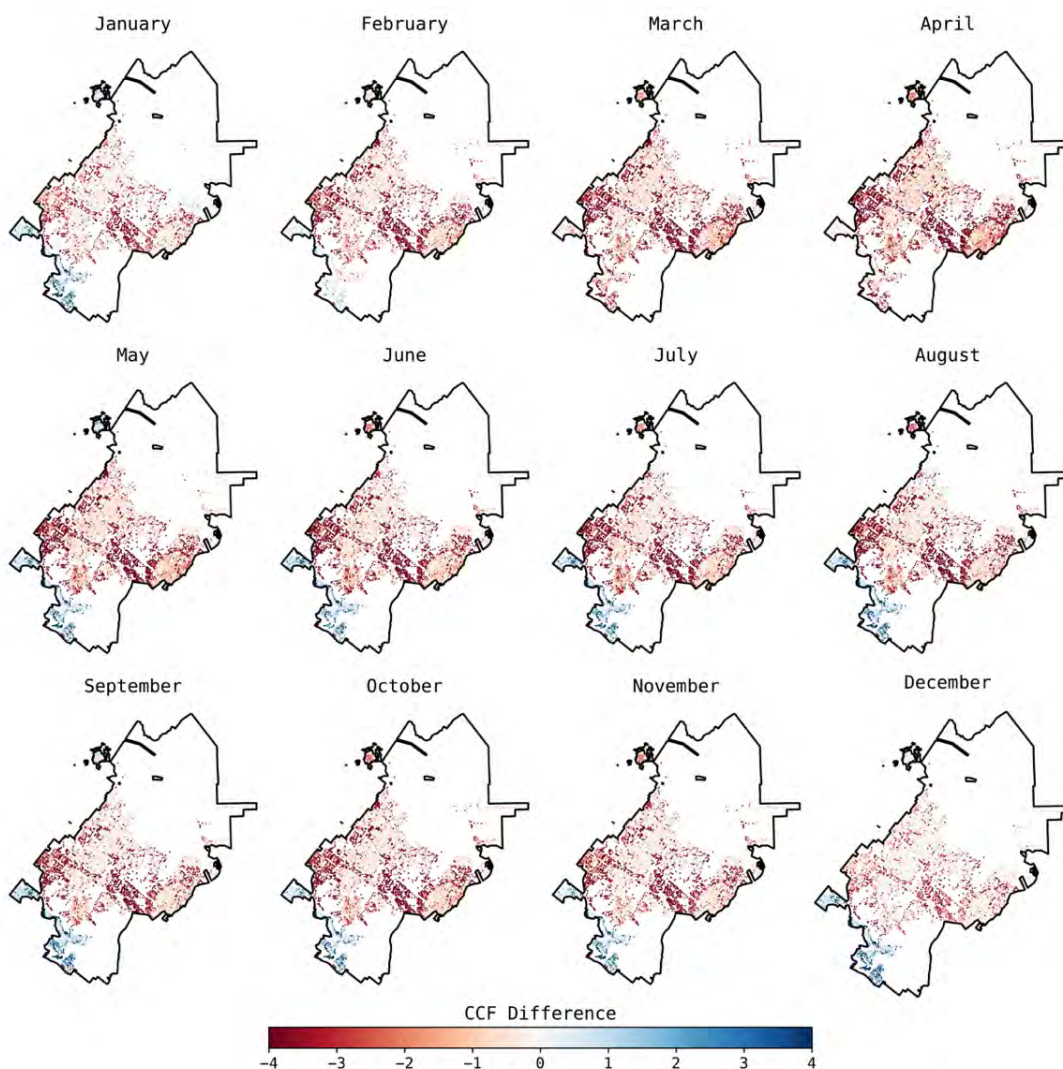
Figure 5. Maps of changes in monthly water budget (in CCF) for each month of the year over the period 2016-2022 when using Spatial CIMIS ETo compared to using IRWD weather stations ETo. Negative (positive) values indicate decreases (increases) in water budget when using Spatial CIMIS.
