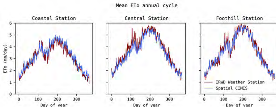
Figure 2. Comparison between the mean daily ETo annual cycle (mm/day) of (brown) the IRWD weather stations and (blue) the Spatial CIMIS at the grid cell co-located with the weather station over the 2016-2022 period.
