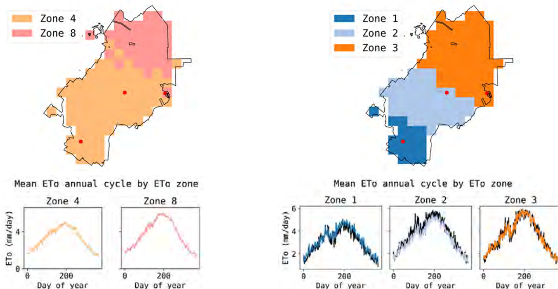
Figure 4. Top left: map of ETo zones for the IRWD based on the California 18 ETo zones map. Bottom left: Mean ETo annual cycle of each ETo zone (zones 4 and 8). Top right: map of ETo zones for the IRWD based on the IRWD 3 ETo zones map. Bottom right: Mean ETo annual cycle of each ETo zone (zones 1 to 3) along with the mean ETo annual cycle of the three IRWD weather stations (black lines). Red dots show the location of the three IRWD weather stations.
