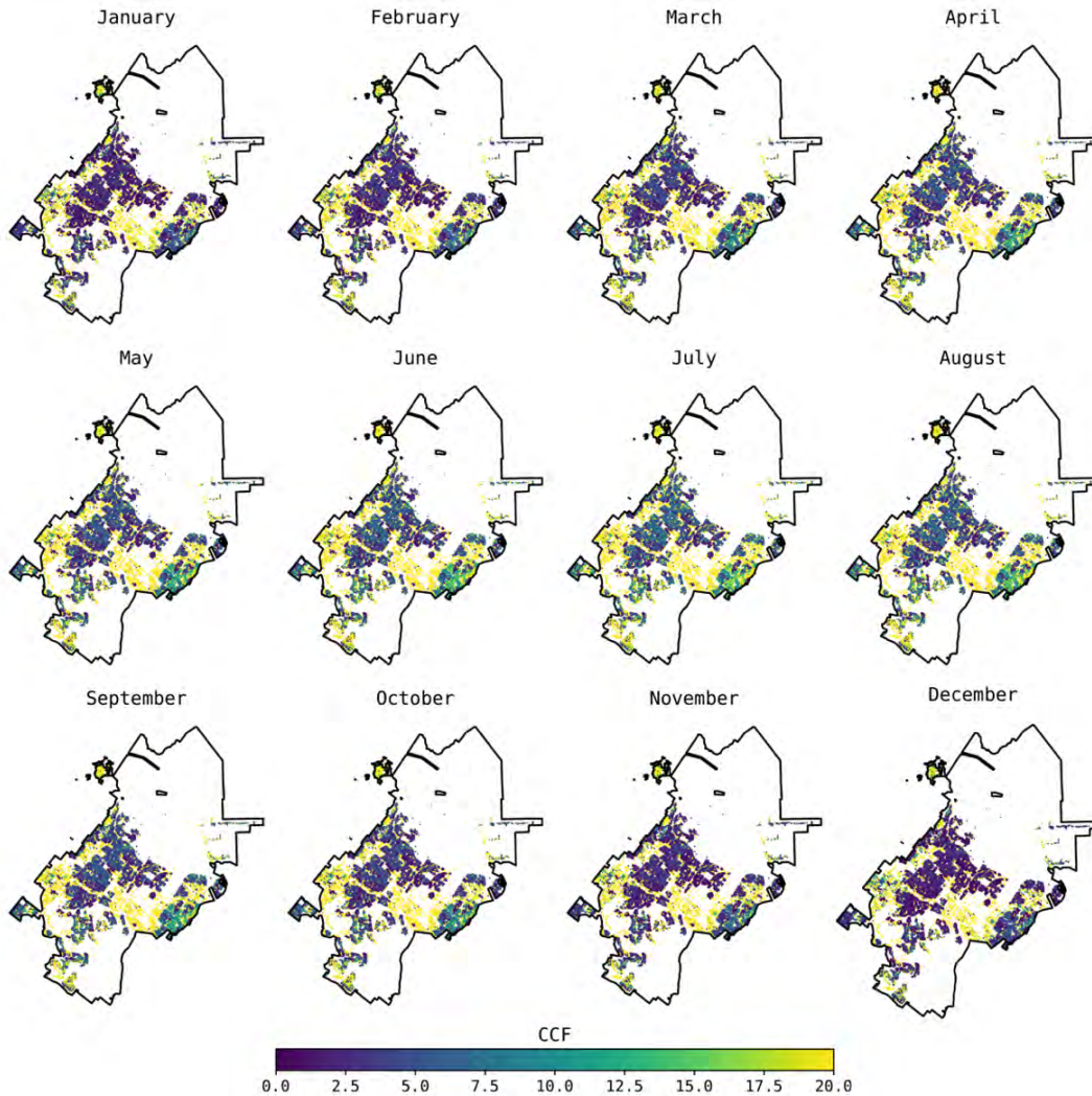
Figure A1. Maps of the water budget (CCF) over the 2016-2022 period computed using the IRWD weather stations ETo.
