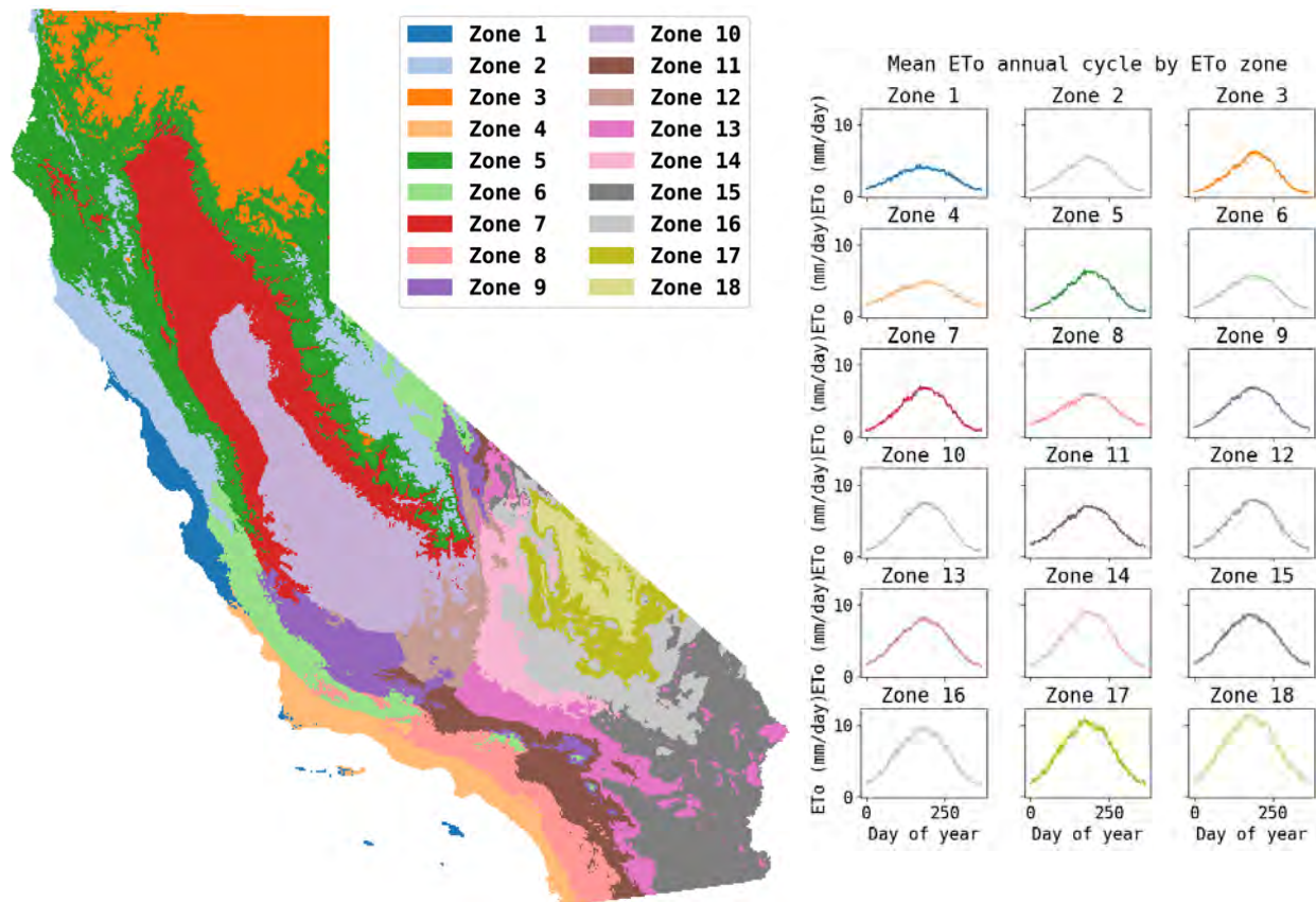
Figure 3. Left: Reference Evapotranspiration (ETo) zones map. Right: Mean ETo annual cycle of each ETo zone. Zones are ordered by the total ETo over the year, with Zone 1 displaying the lowest annual ETo and Zone 18 the high annual ETo.
