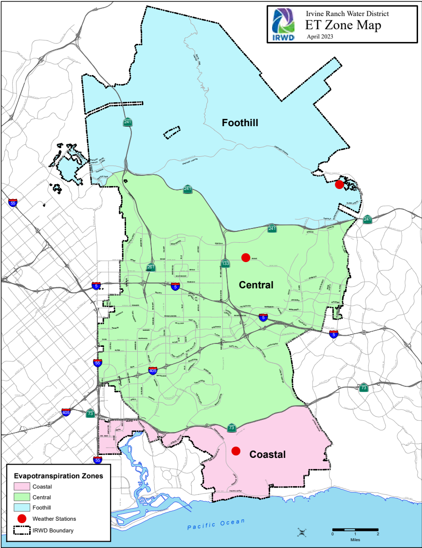
Figure 1. ET zone map for IRWD, dividing the water district into three zones (Coastal, Central and Foothill), and identifying the location of the three IRWD weather stations used to calculate the daily ET for each zone.
