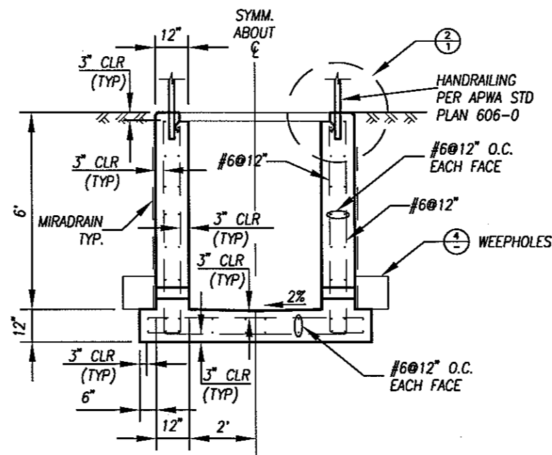
RECTANGULAR CHANNEL SECTION C 1 SCALE: 1" = 4'-0" NOTE: FONTAINE STOP LOGS NOT SHOWN FOR CLARITY.
