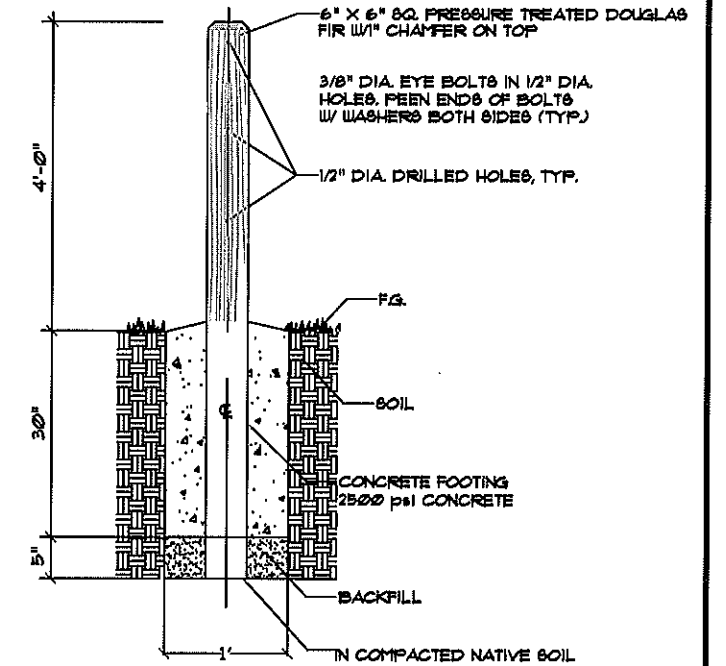
FOOTING DETAIL NTS
