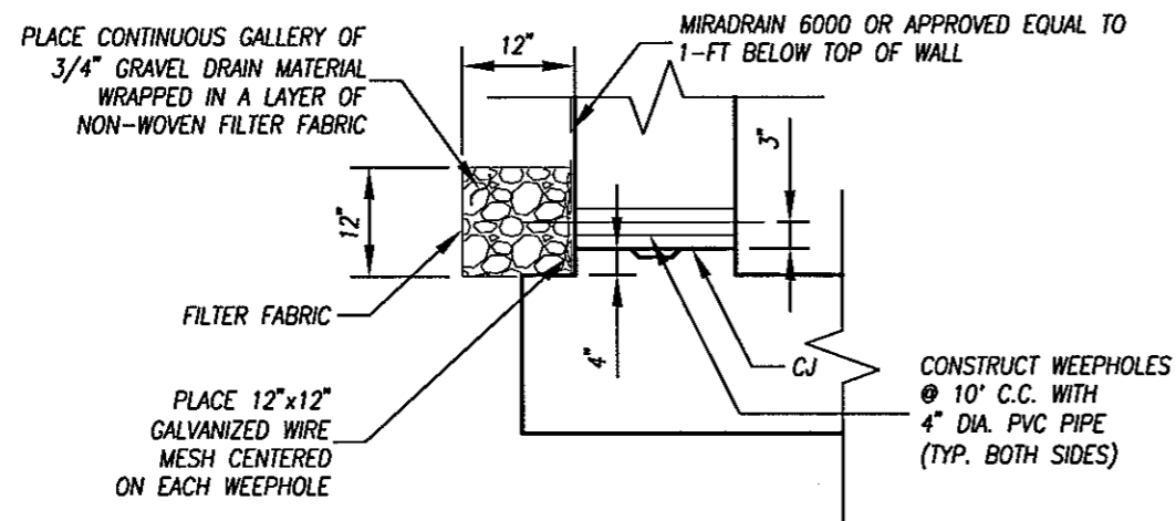
RECT. CHANNEL WEEPHOLE DETAIL 4 N.T.S.
