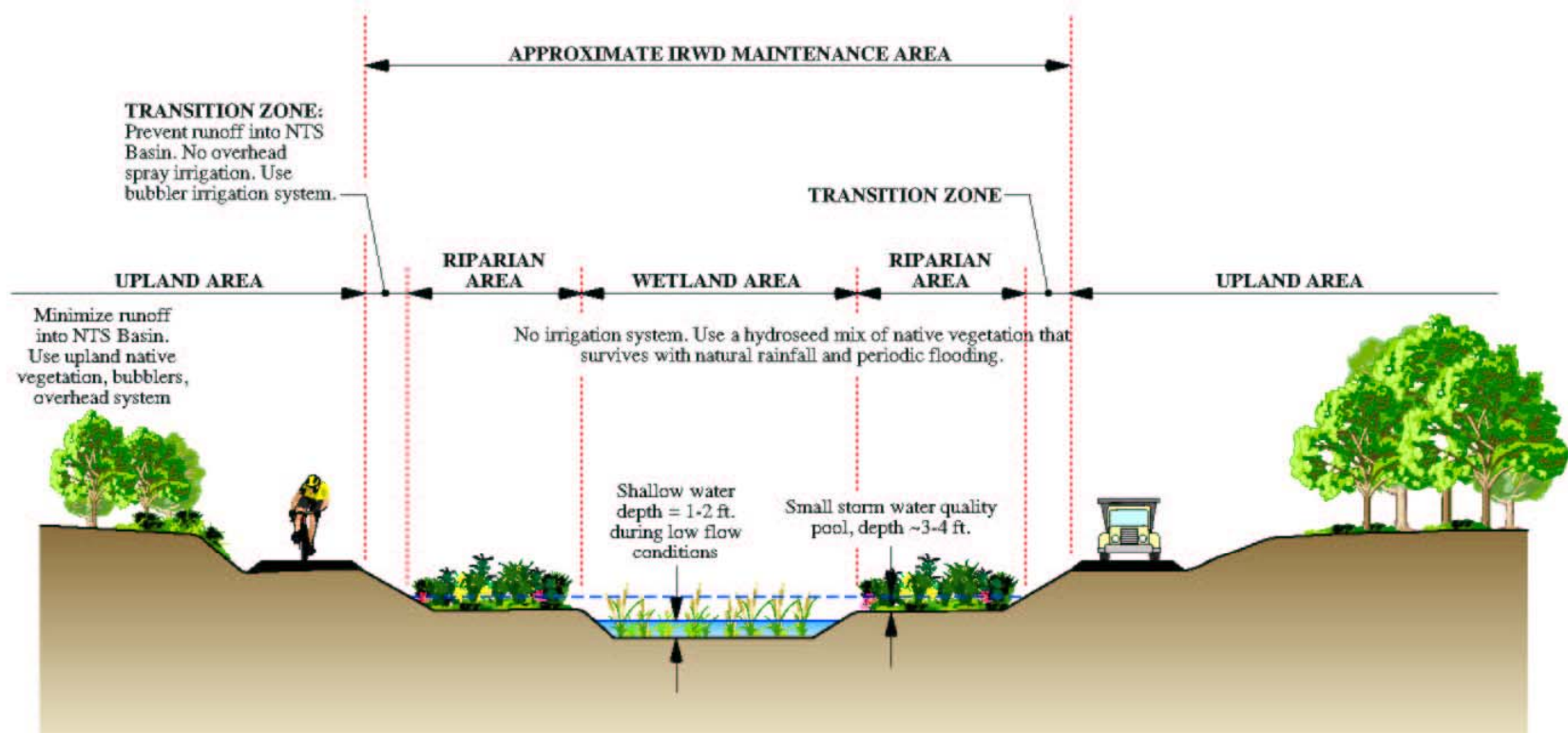
Figure 2 Typical Cross-Section of a Natural Treatment System Showing Vegetation and Irrigation Zones
