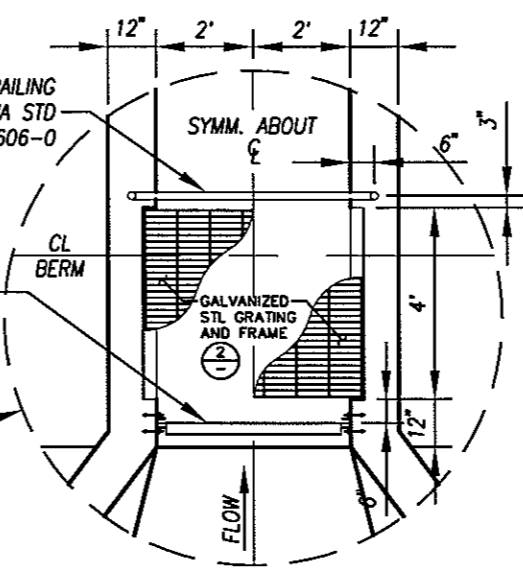
PLAN DETAIL STOP LOG & GRATING SCALE: 1" = 4'-0"
