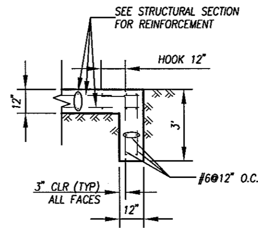
CUTOFF WALL 5 1 SCALE: 1" = 4'-0"
